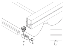
F3 Slider & Fabric Profile Assembly The system has been designed for ease of assembly to save time on installations and reduce the number of staff required.
