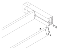
Motorbox Support & Hood Support Profile Easy Installation Each support profile is easy to install and simple to adjust at time of installation.
