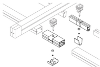
Easy Clip Intermediate Joints (2&3 module) The easy clip intermediate joints have been designed for ease of site assembly to save time and reduce the number of staff required..
