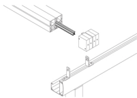
Storm Channel For Joining System The storm channel is a patented solution for joining two systems side by side with a waterproof join.
