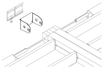
Double Rafter Wall Bracket Kit An advanced solution for installing two rafters at once.
