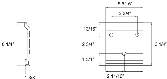
Installation Bracket
