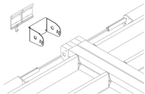
Double Rafter Wall Bracket Kit An advanced solution for installing two rafters at once.
