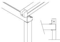
Rafter Profile Joining Piece Gutter solution for when the system is installed next to a wall or no overhang of the gutter is required..
