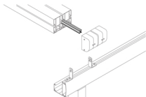
Storm Channel For Joining System The storm channel is a patented solution for joining two systems side by side with a waterproof join.
